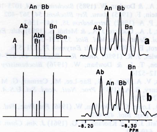
FIGURE 2: ^{31}\text{P} NMR analyses of [\text{}^{17}\text{O}, \text{}^{18}\text{O}] DPPE from the product of the reactions catalyzed by E. coli PS synthase (coupled with PS decarboxylase): (a) from 1a ; (b) from 1b . Spectral conditions were similar to those of Figure 1. The calculated spectra (left) were obtained with 100% retention of the configuration for PS synthase.
